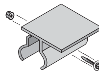
Standing-seam clamp
